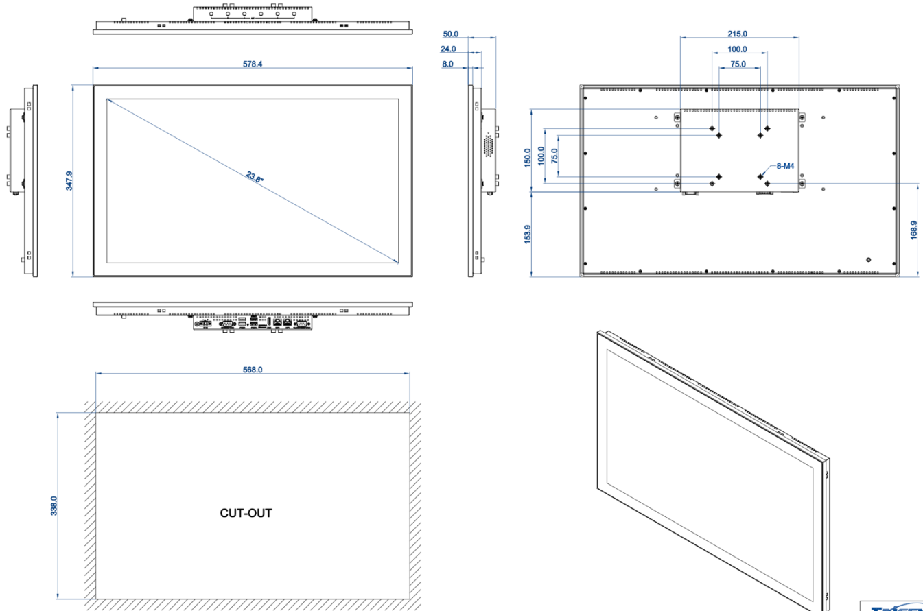
DIMENSIONAL DRAWING:TPC-DCS238R2
