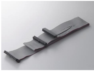
P/N 1700340640 FDD cable for two 3.5" FDD
