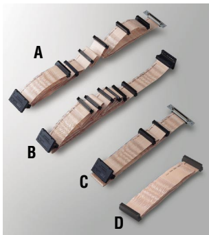
A. P/N 1701681790 68-pin SCSI LVDS cable, F-6M-T, 179 cm, for RAID-500U3 B. P/N 1701681560 68-pin SCSI LVDS cable, T-6M-T, 156 cm C. P/N 1701681100 68-pin SCSI LVDS cable, F-M-M-T, 110 cm D. P/N 1701680550 68-pin SCSI LVDS cable, F-M-M-T, 53 cm
