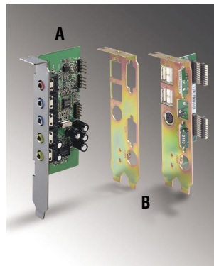
A. P/N PCA-AUDIO-00A1 Audio extension module (AC-97) provides Line-in, MIC-in, Aux-in, Line-out, Speaker-out, CD-in and Buzzer-in from CPU card B. P/N PCA-USB4-00A1 USB extension module with 4 ports
