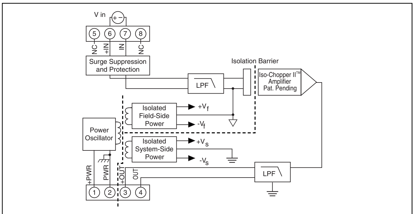
Fig 1: DSCA40/41 Block Diagram
