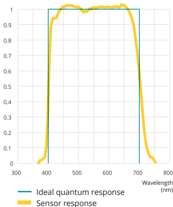
Typical quantum response
